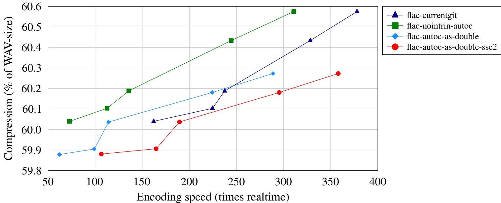
Encoding realtime speed vs compression for check-autoc-sse2-intrinsics
