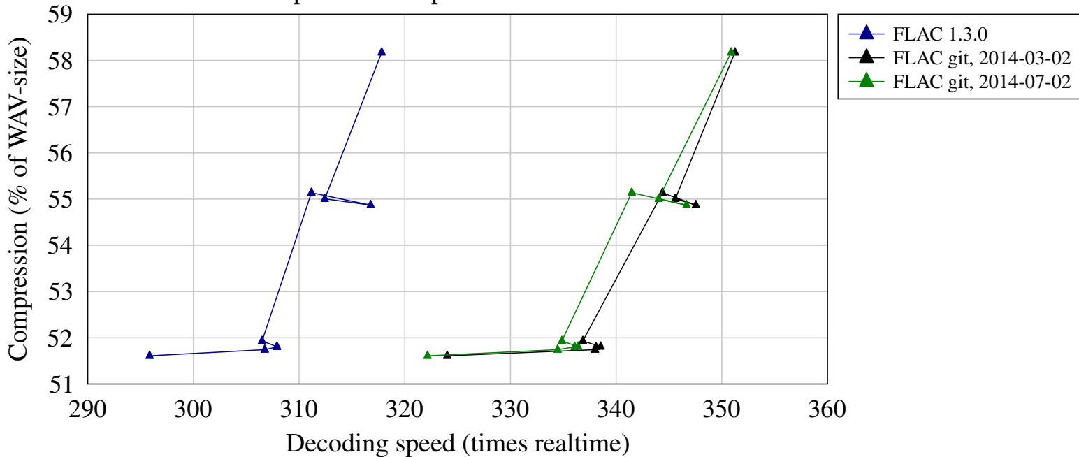
Decoding speed vs compression for short set of samples - FLAC performance test - Wine MSVC 2013
