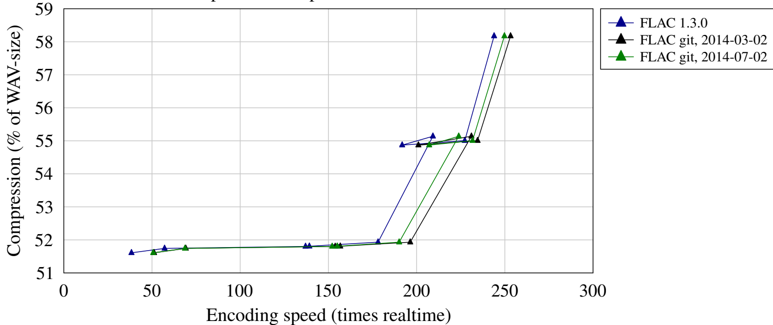
Encoding speed vs compression for short set of samples - FLAC performance test - Wine MSVC 2013
