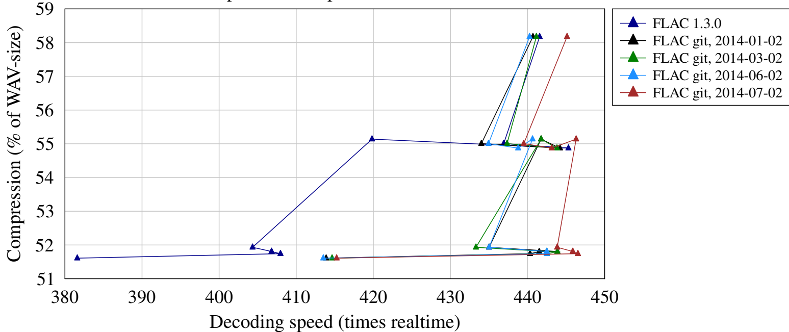
Decoding speed vs compression for short set of samples - FLAC performance test - Linux GCC 4.8
