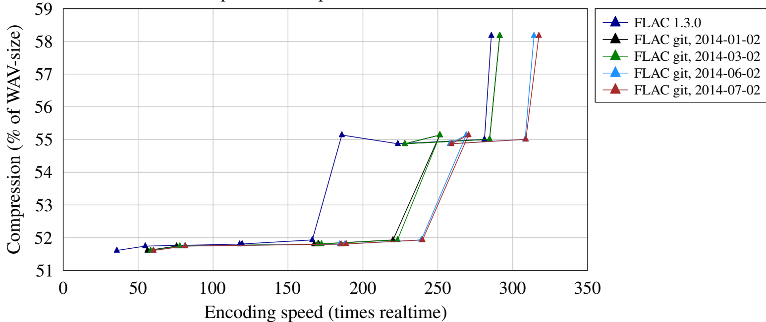
Encoding speed vs compression for short set of samples - FLAC performance test - Linux GCC 4.8
